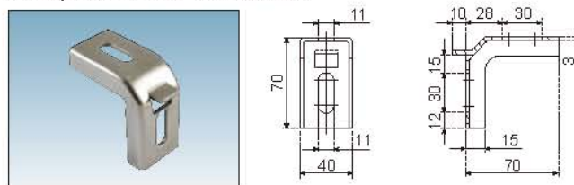
带钩L型不锈钢钣金支架 L Shape With Hook SS Brackets
