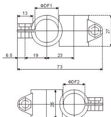
N202T 十字承夹 N202T Cross Clamps
