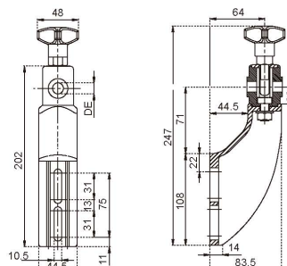
N241B 护栏支架 N241B Side Guide Brackets
