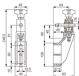
N238 护栏支架 N238 Side Guide Brackets
