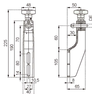
N239 护栏支架 N239 Side Guide Brackets
