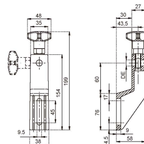
N240B 护栏支架 N240B Side Guide Brackets
