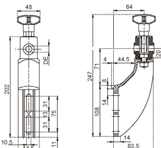
N241A 护栏支架 N241A Side Guide Brackets
