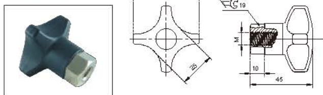
N234A 旋紧头 N234A Knobs
