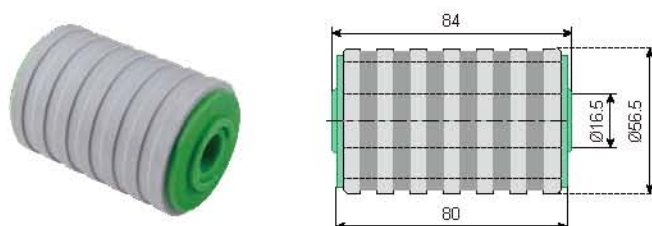
N454 带胶防水托轮 N454 Watertight Roller with Rubber
