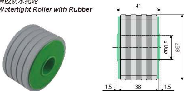
N453 带胶防水托轮 N453 Watertight Roller with Rubber
