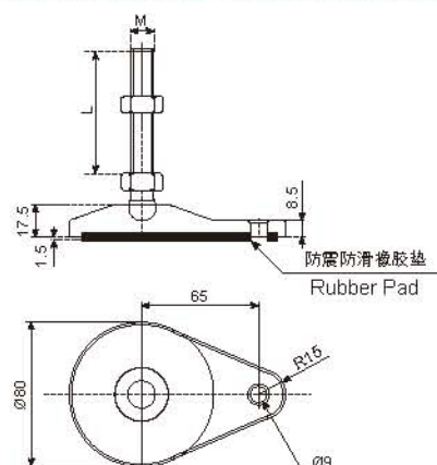
D80C 万向关节调整脚踏 D80C Articulated feet
