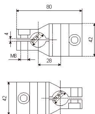
N202SS-2 十字承夹 N202SS-2 Cross Clamps
