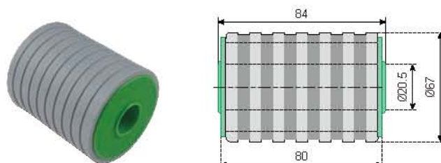
N453 带胶防水托轮 N453 Watertight Roller with Rubber
