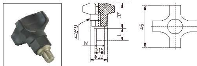
N235C 旋紧头 N235C Knobs
