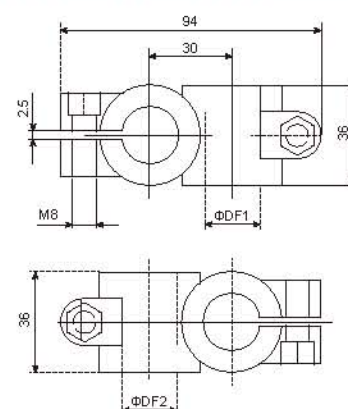
N202SS-1 十字承夹 N202SS-1 Cross Clamps
