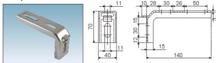
带钩L型不锈钢钣金支架 L Shape With Hook SS Brackets
