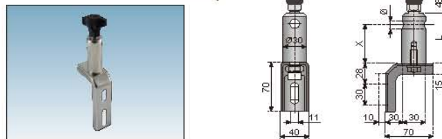
不锈钢钣金支架调整组 SS Brackets Articulated Group
